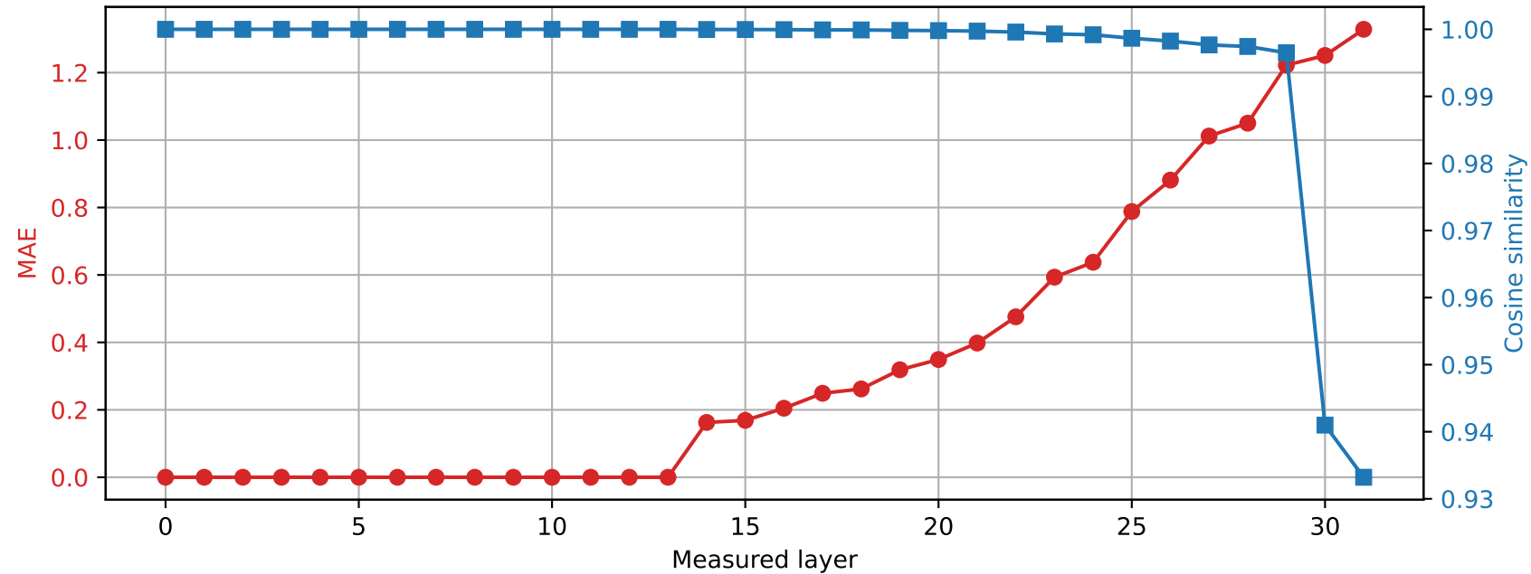
Phi-3-mini-4k-instruct | Prompt 4 Spared layer 13 | Hybrid vs quantized
