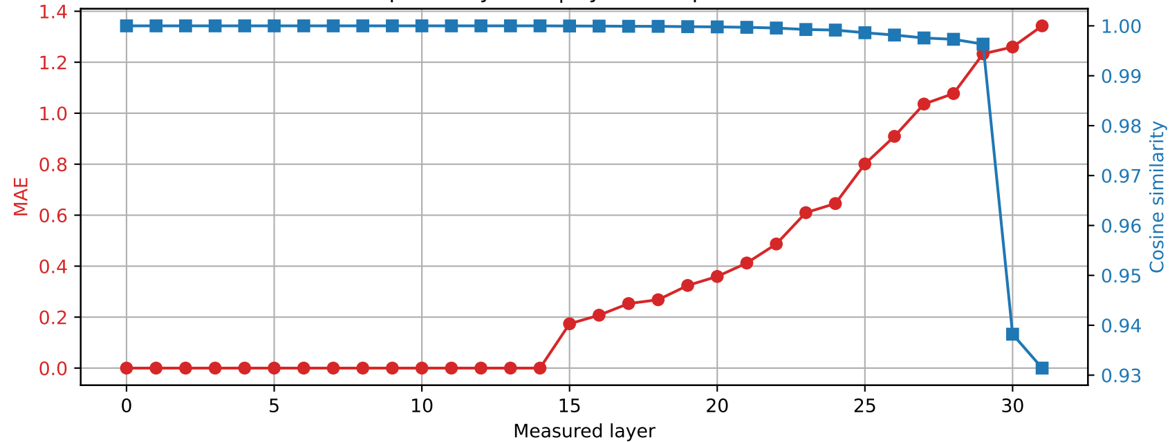
Phi-3-mini-4k-instruct | Prompt 4 Spared layer 14 | Hybrid vs quantized
