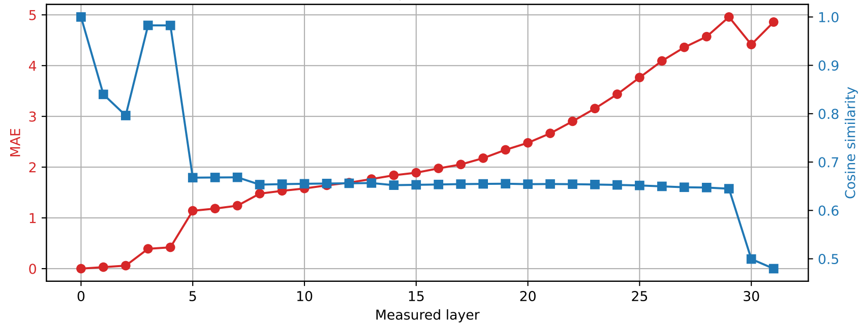
Phi-3-mini-4k-instruct | Prompt 4 Spared layer 16 | Hybrid vs unquantized
