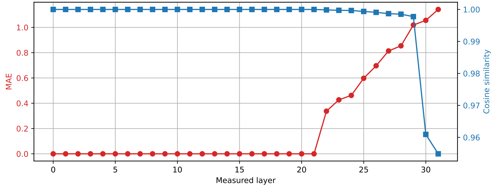
Phi-3-mini-4k-instruct | Prompt 4 Spared layer 21 | Hybrid vs quantized
