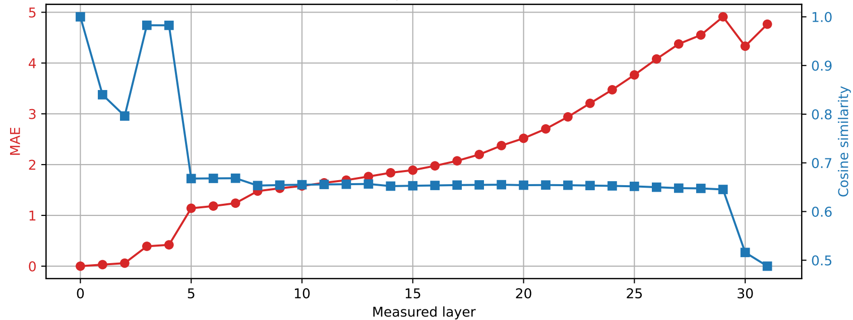
Phi-3-mini-4k-instruct | Prompt 4 Spared layer 24 | Hybrid vs unquantized
