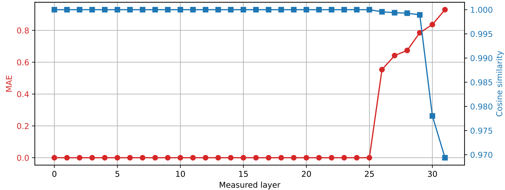
Phi-3-mini-4k-instruct | Prompt 4 Spared layer 25 | Hybrid vs quantized
