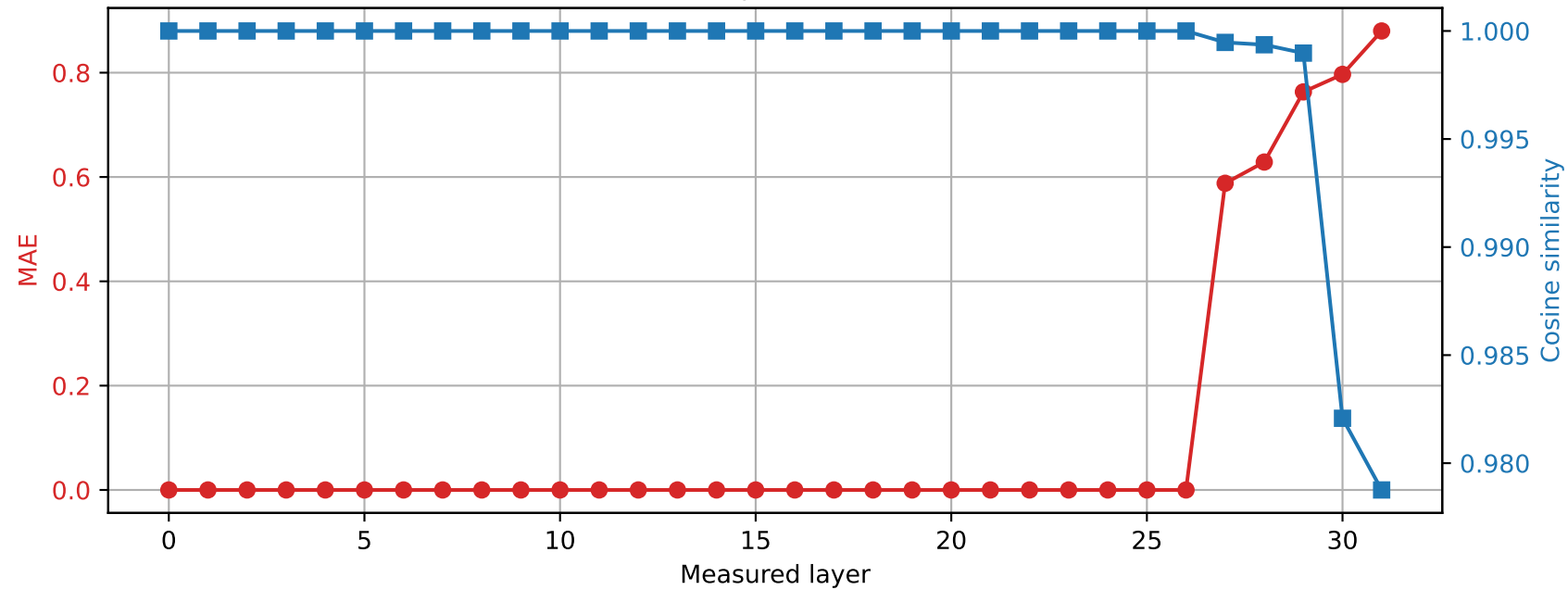
Phi-3-mini-4k-instruct | Prompt 4 Spared layer 26 | Hybrid vs quantized
