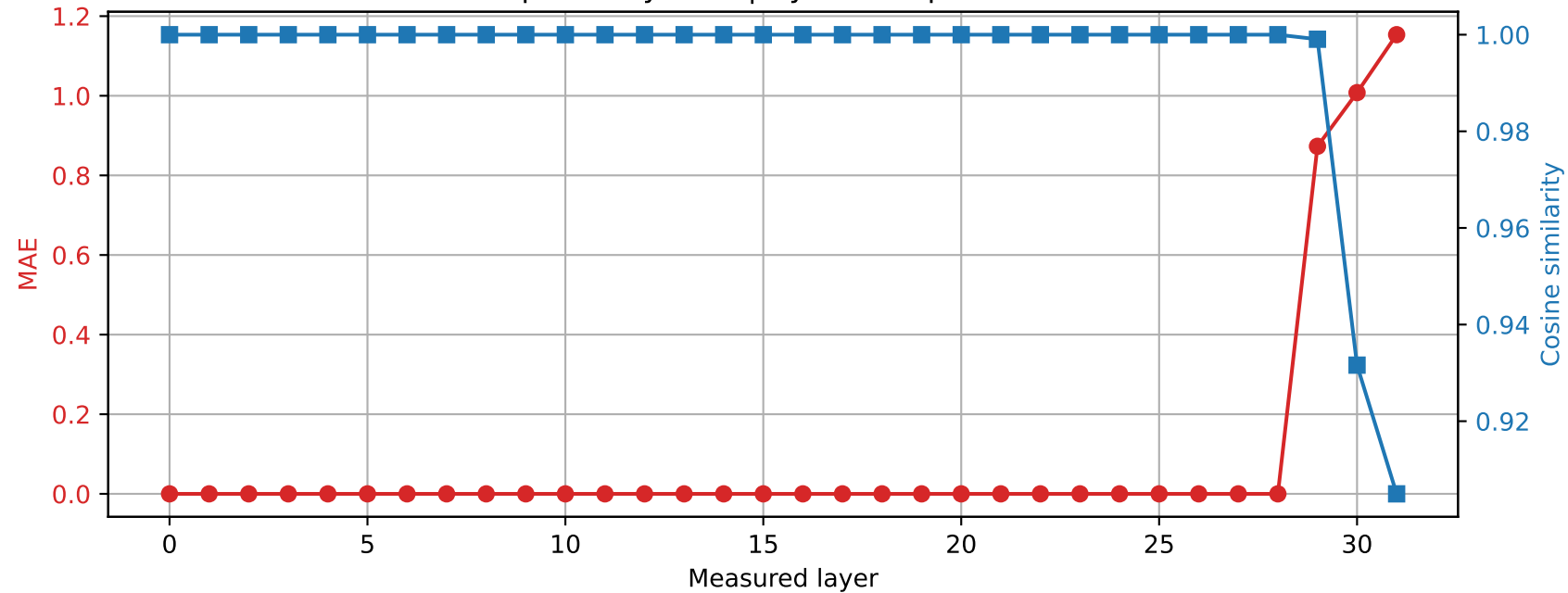
Phi-3-mini-4k-instruct | Prompt 4 Spared layer 28 | Hybrid vs quantized
