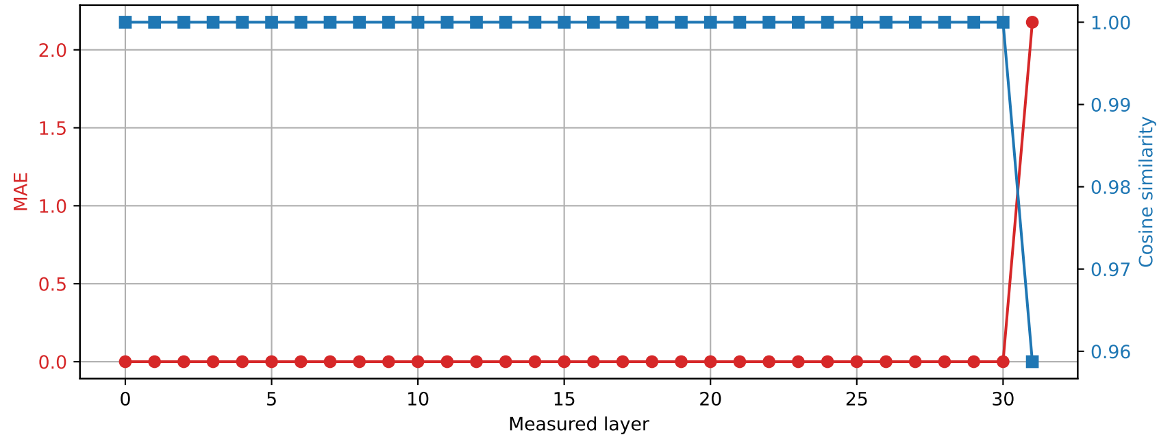
Phi-3-mini-4k-instruct | Prompt 4 Spared layer 30 | Hybrid vs quantized
