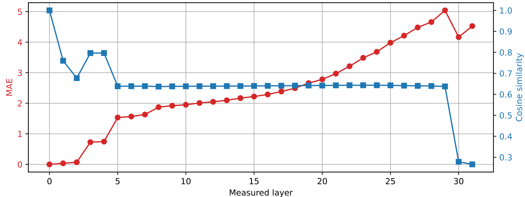
Phi-3-mini-4k-instruct | Prompt 0 Spared layer 2 | Hybrid vs unquantized
