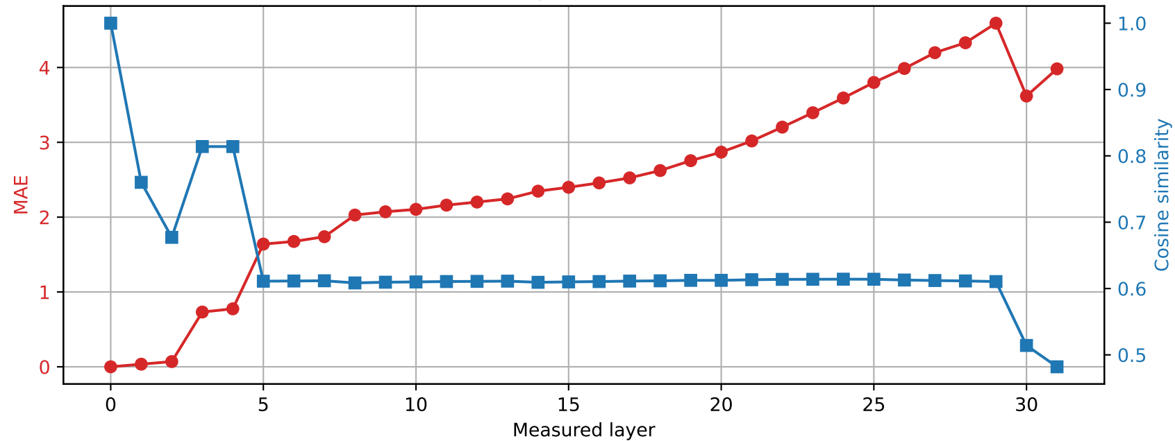
Phi-3-mini-4k-instruct | Prompt 0 Spared layer 3 | Hybrid vs unquantized
