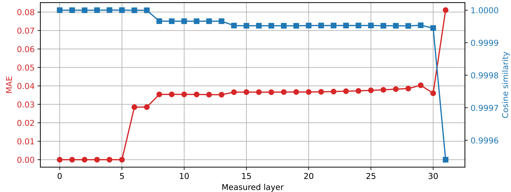
Phi-3-mini-4k-instruct | Prompt 0 Spared layer 5 | Hybrid vs quantized
