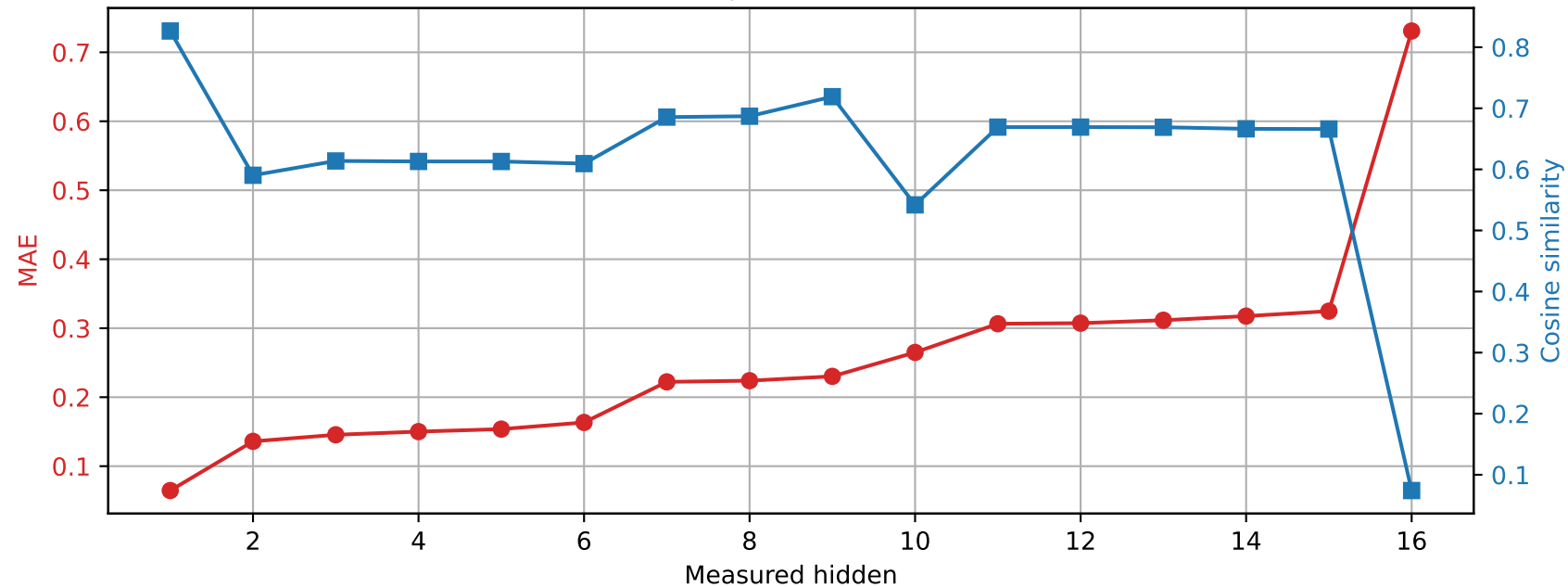
OLMo-1B-hf | Prompt 0 Spared layer 6 | Unquantized vs hybrid
