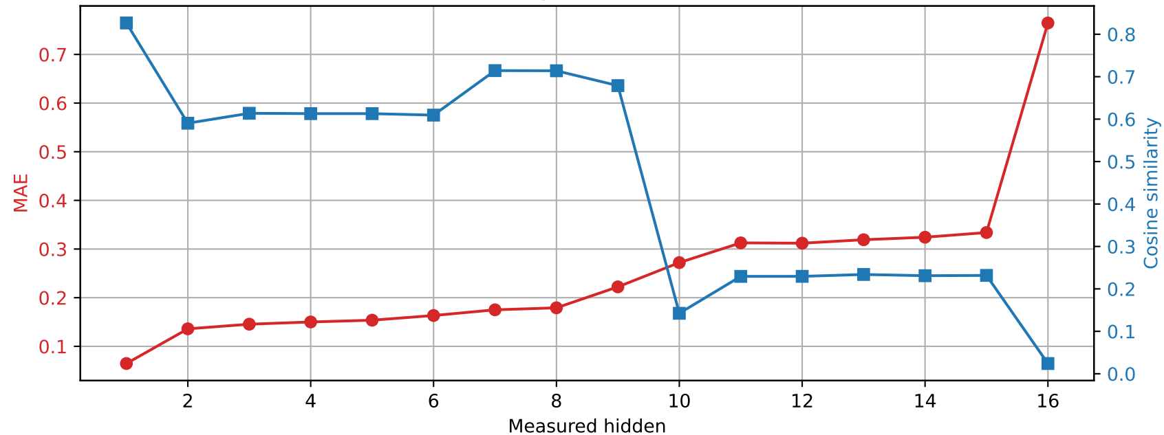
OLMo-1B-hf | Prompt 0 Spared layer 8 | Unquantized vs hybrid
