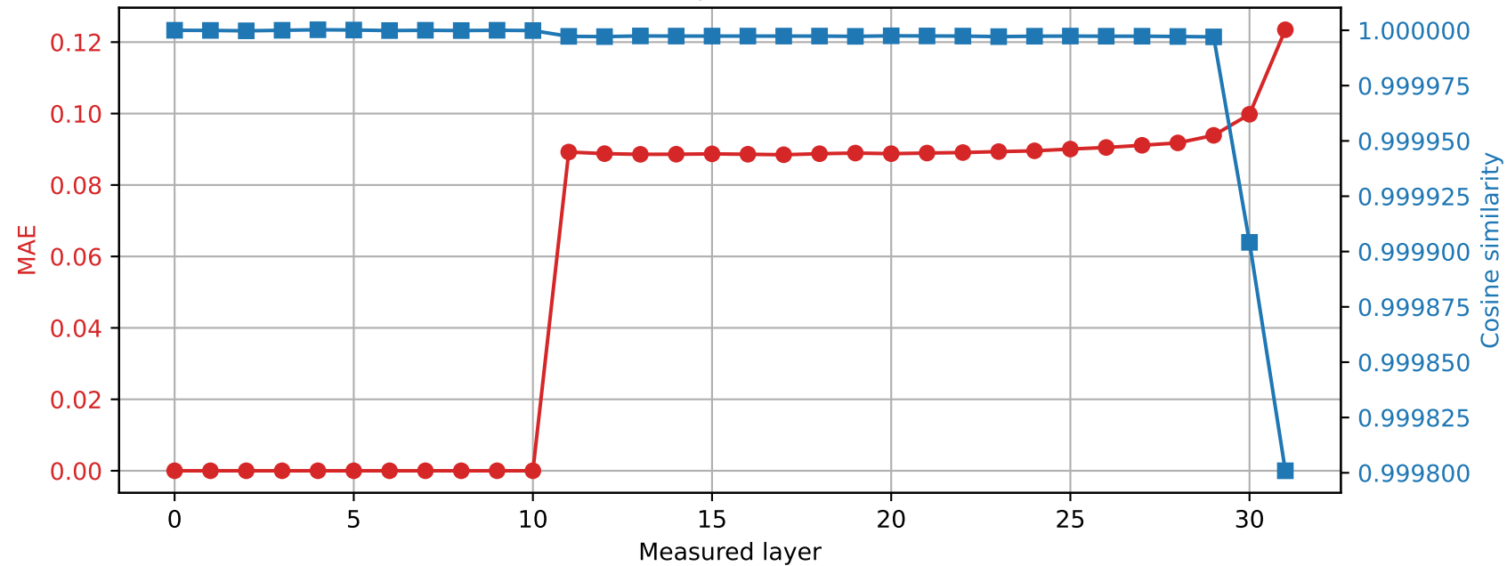
Phi-3-mini-4k-instruct | Prompt 0 Spared layer 10 | Hybrid vs quantized
