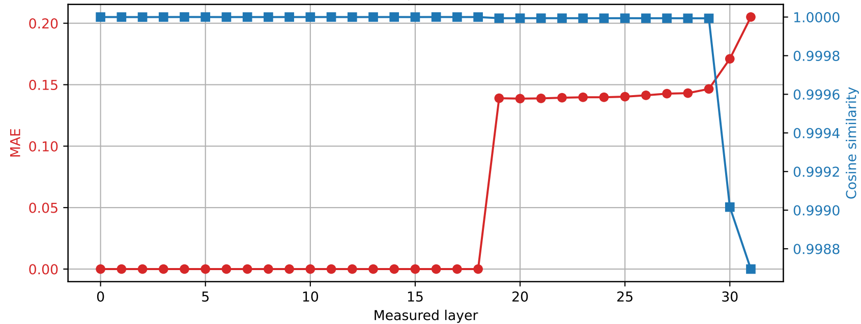
Phi-3-mini-4k-instruct | Prompt 0 Spared layer 18 | Hybrid vs quantized
