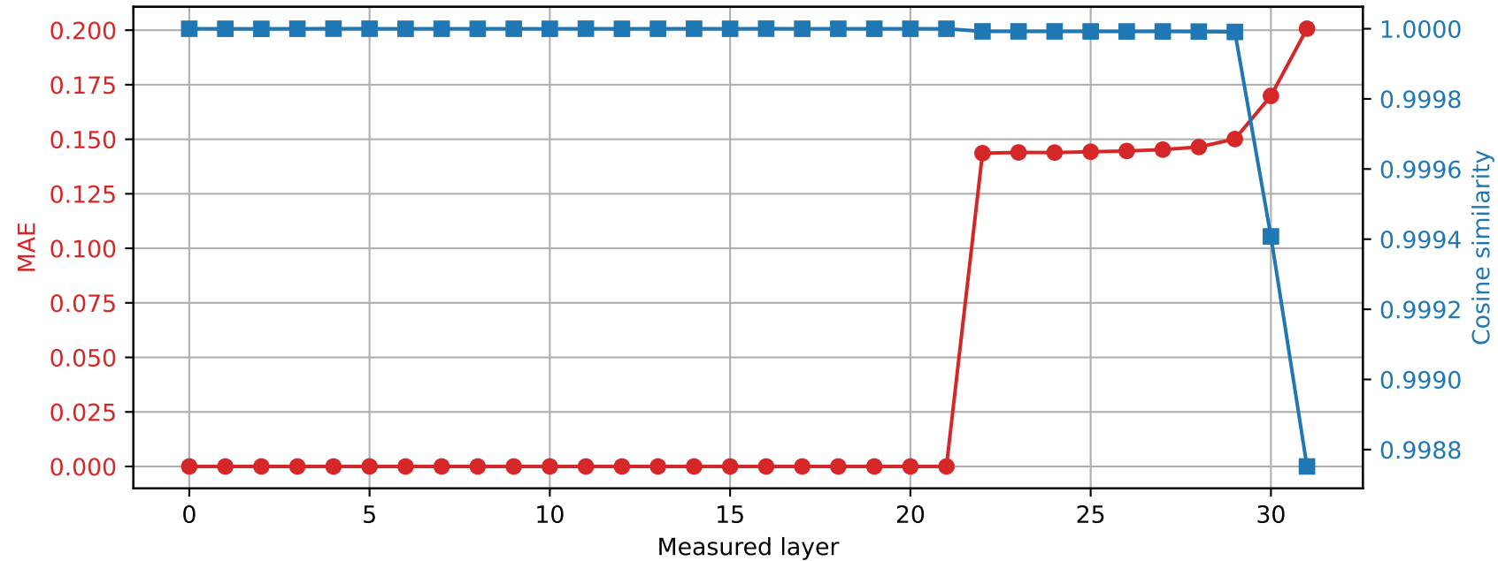
Phi-3-mini-4k-instruct | Prompt 0 Spared layer 21 | Hybrid vs quantized
