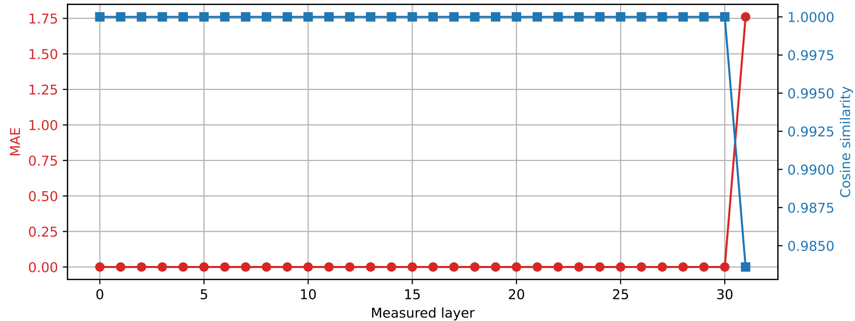
Phi-3-mini-4k-instruct | Prompt 0 Spared layer 30 | Hybrid vs quantized
