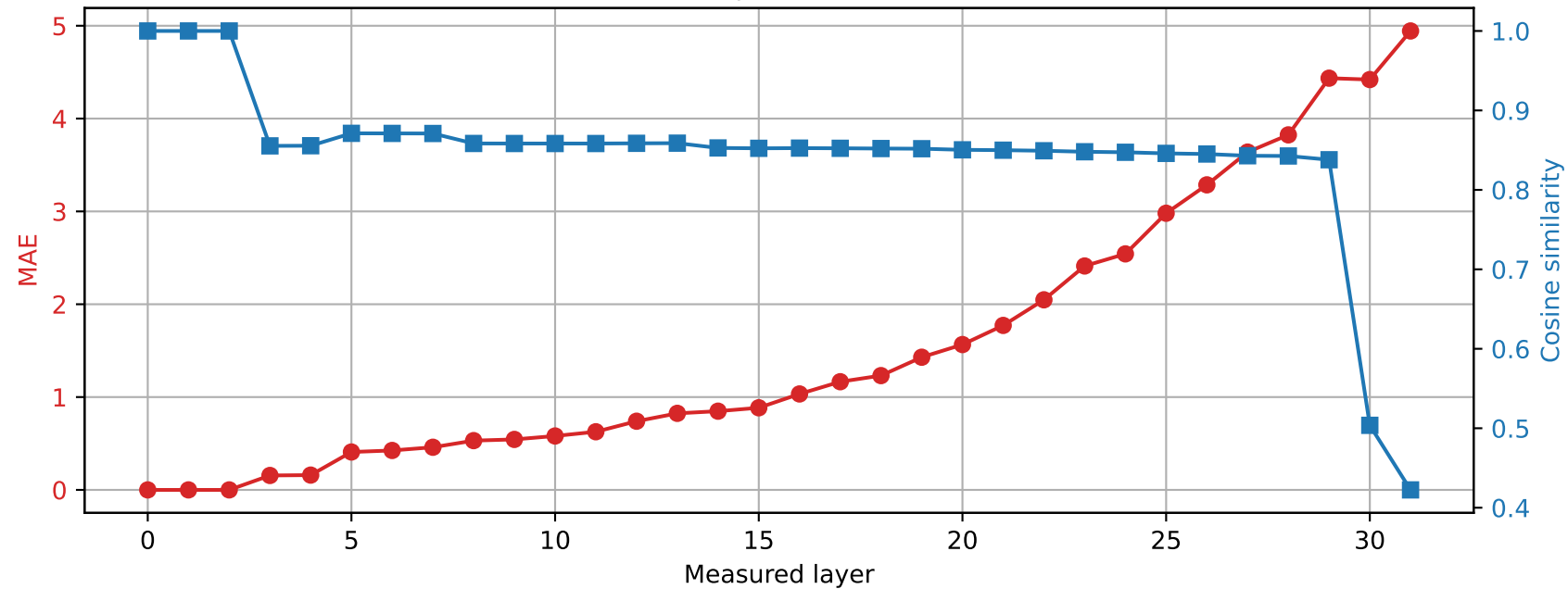
Phi-3-mini-4k-instruct | Prompt 1 Spared layer 2 | Hybrid vs quantized
