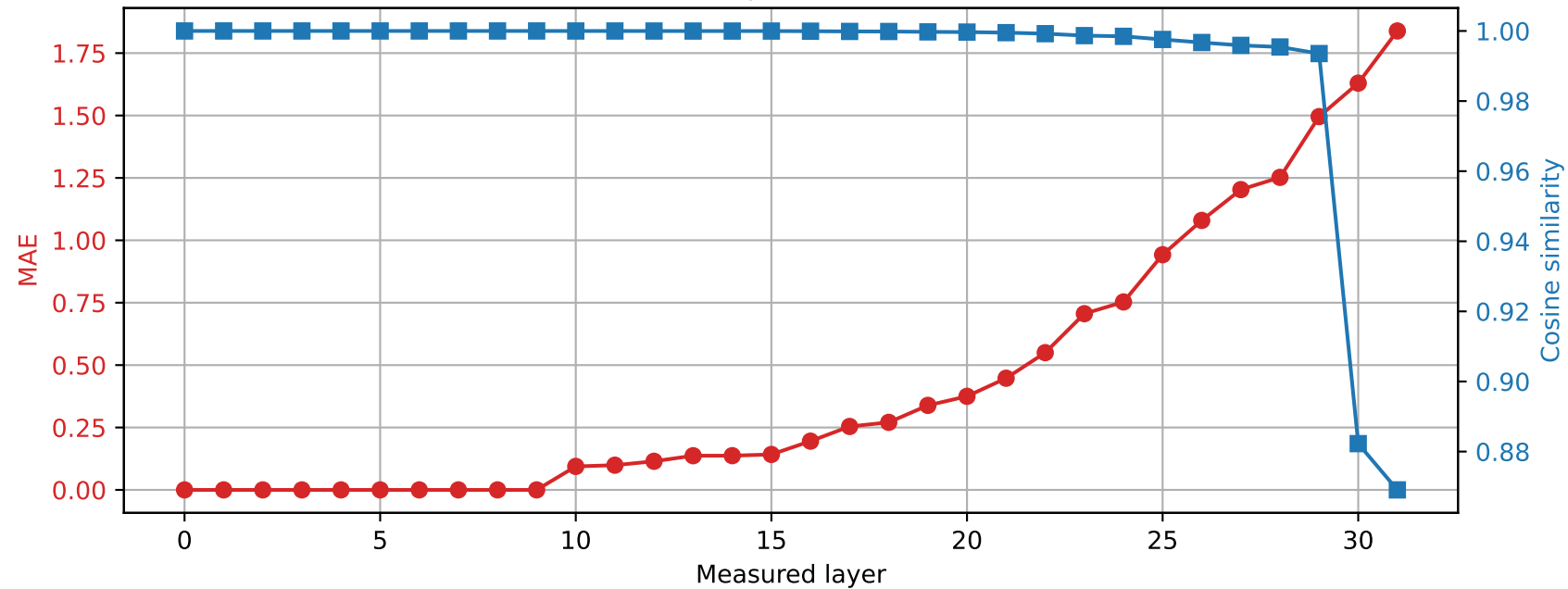
Phi-3-mini-4k-instruct | Prompt 1 Spared layer 9 | Hybrid vs quantized
