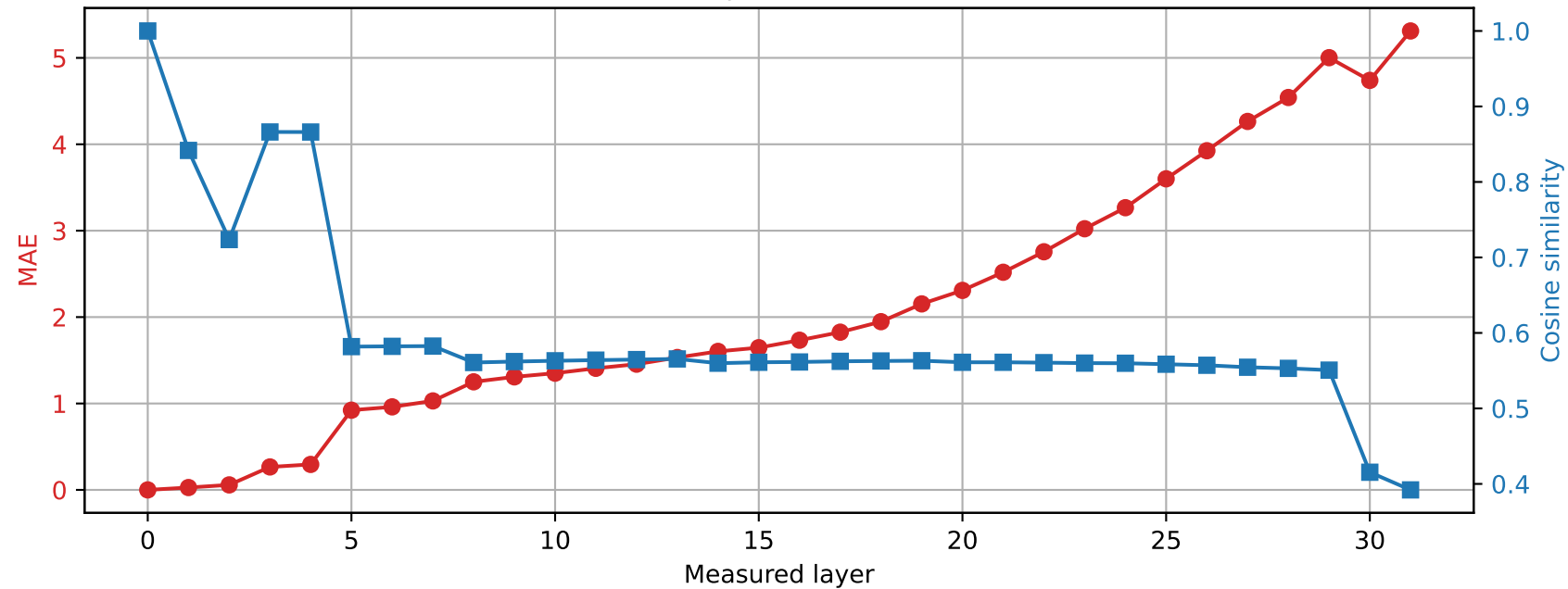
Phi-3-mini-4k-instruct | Prompt 1 Spared layer 11 | Hybrid vs unquantized
