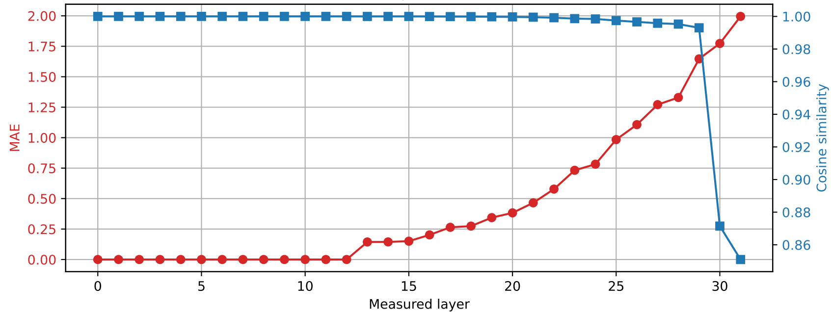
Phi-3-mini-4k-instruct | Prompt 1 Spared layer 12 | Hybrid vs quantized
