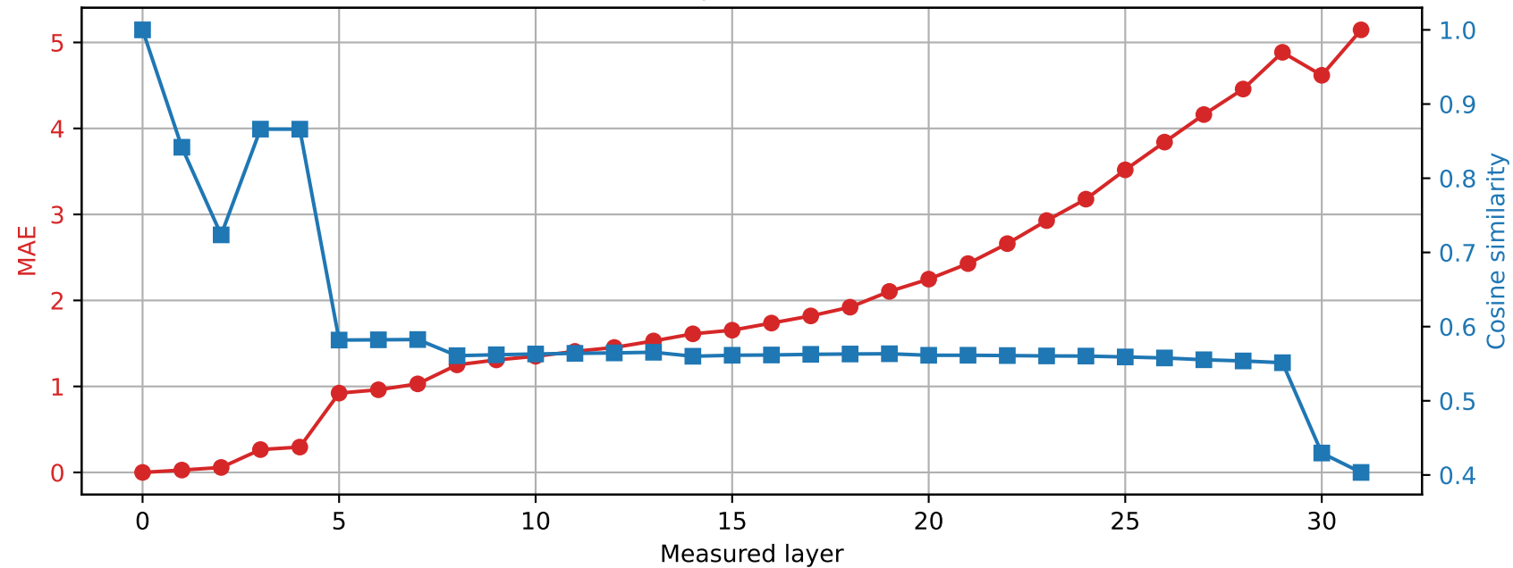
Phi-3-mini-4k-instruct | Prompt 1 Spared layer 13 | Hybrid vs unquantized
