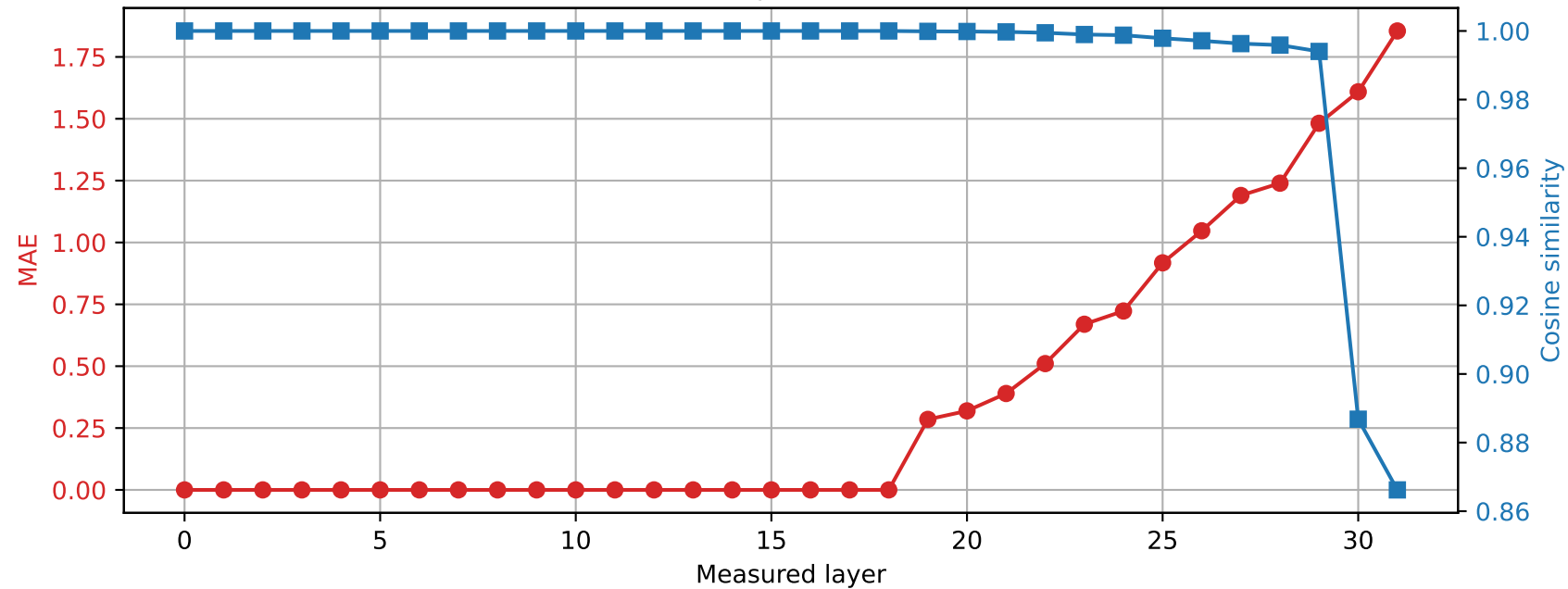
Phi-3-mini-4k-instruct | Prompt 1 Spared layer 18 | Hybrid vs quantized
