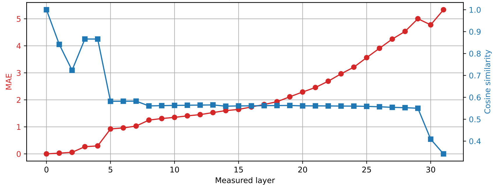
Phi-3-mini-4k-instruct | Prompt 1 Spared layer 19 | Hybrid vs unquantized
