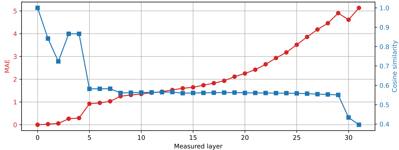
Phi-3-mini-4k-instruct | Prompt 1 Spared layer 20 | Hybrid vs unquantized
