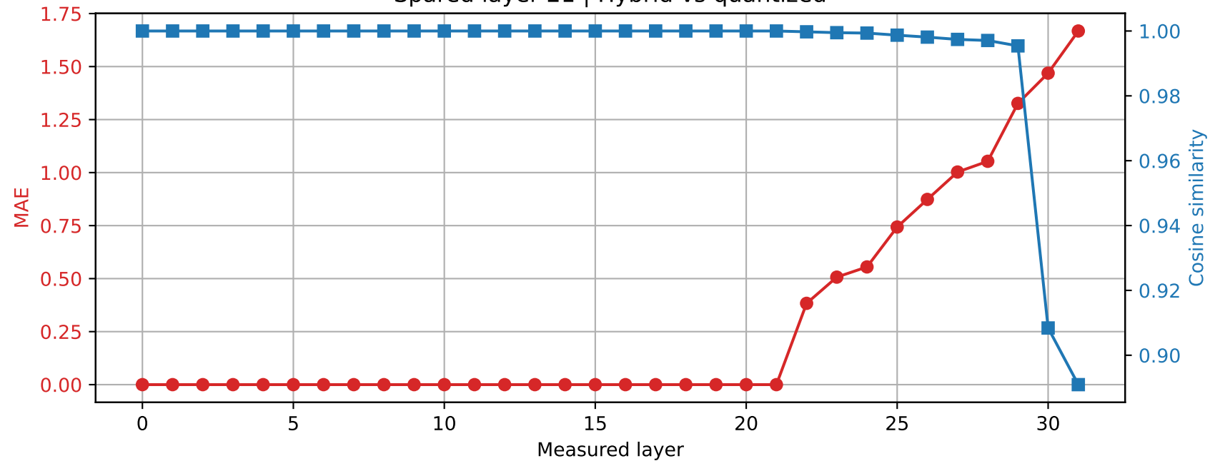
Phi-3-mini-4k-instruct | Prompt 1 Spared layer 21 | Hybrid vs quantized
