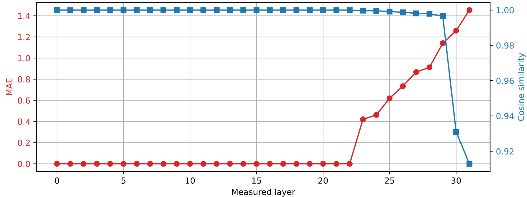
Phi-3-mini-4k-instruct | Prompt 1 Spared layer 22 | Hybrid vs quantized
