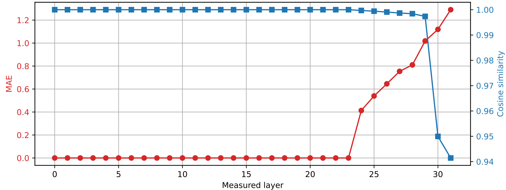
Phi-3-mini-4k-instruct | Prompt 1 Spared layer 23 | Hybrid vs quantized
