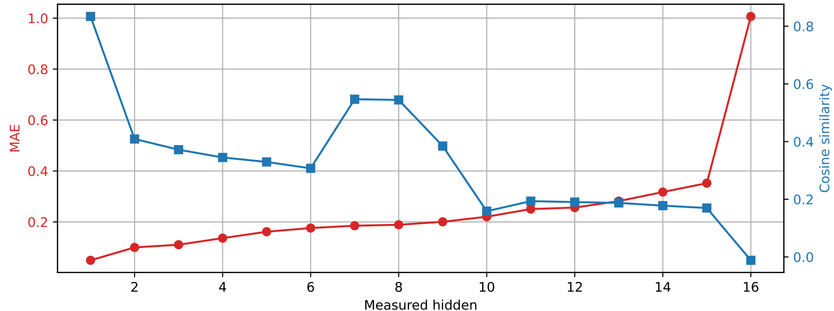
OLMo-1B-hf | Prompt 2 Spared layer 3 | Unquantized vs hybrid
