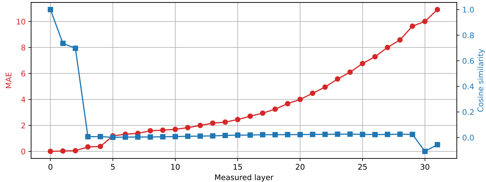
Phi-3-mini-4k-instruct | Prompt 2 Spared layer 5 | Hybrid vs unquantized
