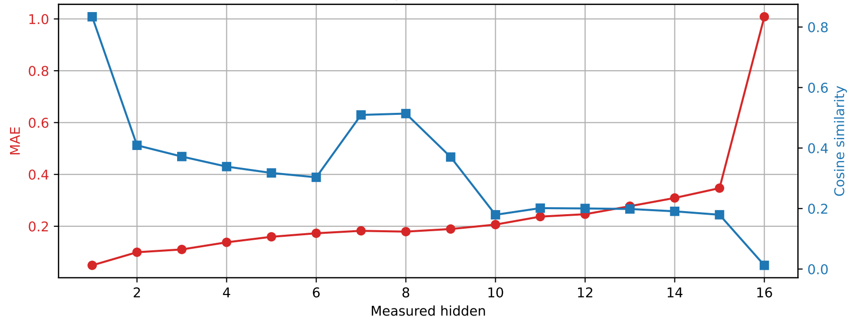
OLMo-1B-hf | Prompt 2 Spared layer 7 | Unquantized vs hybrid
