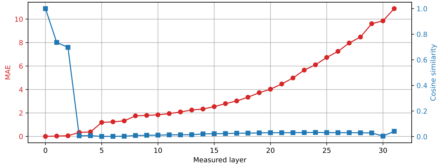
Phi-3-mini-4k-instruct | Prompt 2 Spared layer 7 | Hybrid vs unquantized
