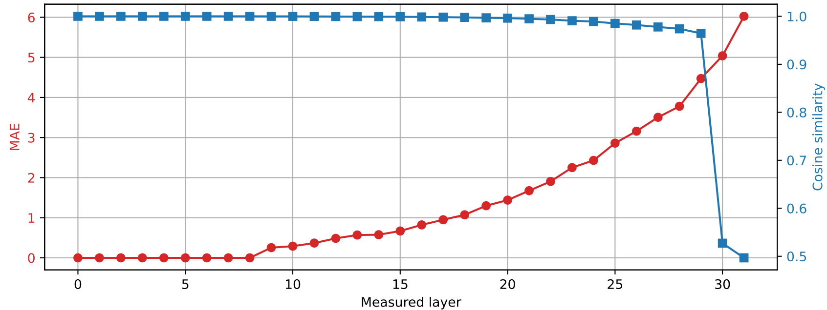
Phi-3-mini-4k-instruct | Prompt 2 Spared layer 8 | Hybrid vs quantized
