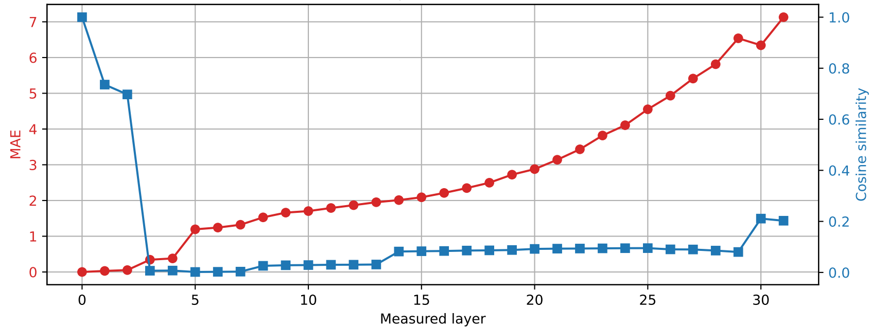
Phi-3-mini-4k-instruct | Prompt 2 Spared layer 8 | Hybrid vs unquantized
