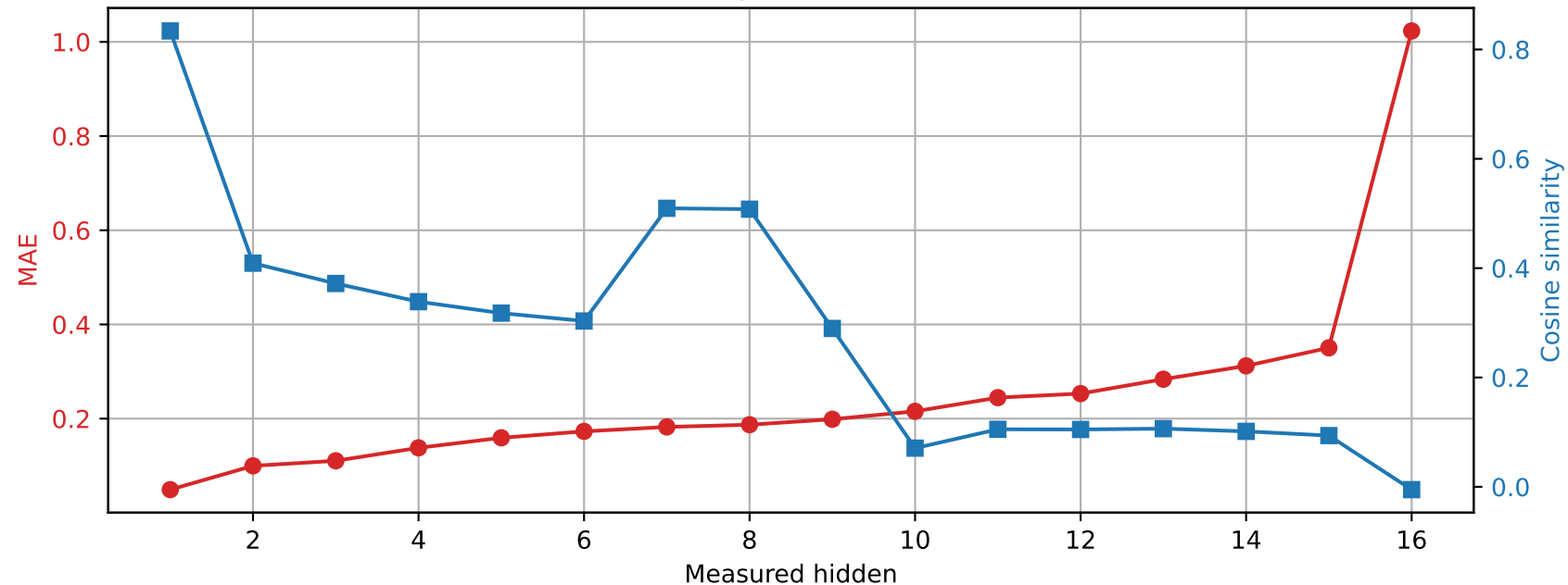
OLMo-1B-hf | Prompt 2 Spared layer 13 | Unquantized vs hybrid
