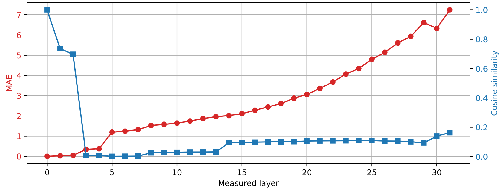
Phi-3-mini-4k-instruct | Prompt 2 Spared layer 23 | Hybrid vs unquantized
