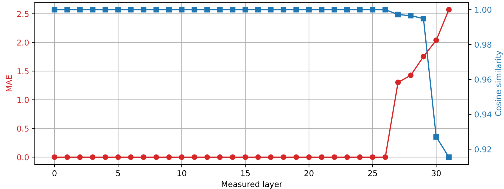
Phi-3-mini-4k-instruct | Prompt 2 Spared layer 26 | Hybrid vs quantized
