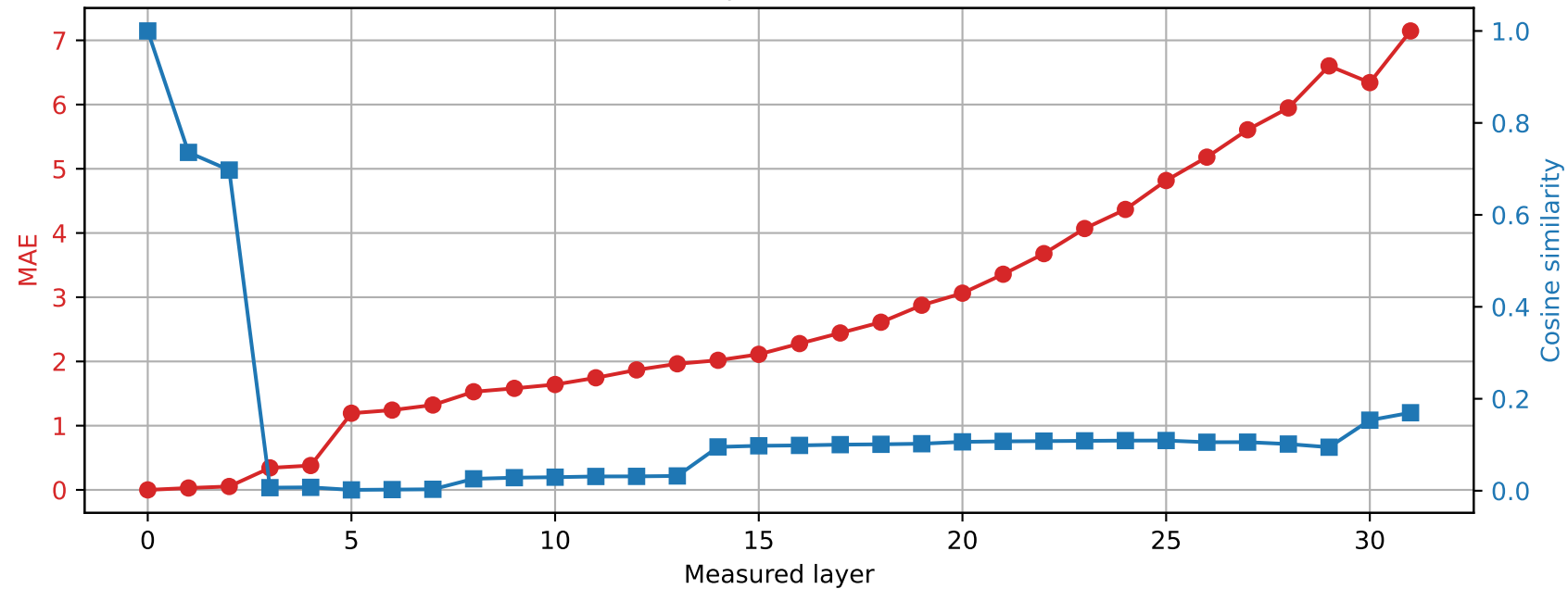
Phi-3-mini-4k-instruct | Prompt 2 Spared layer 26 | Hybrid vs unquantized
