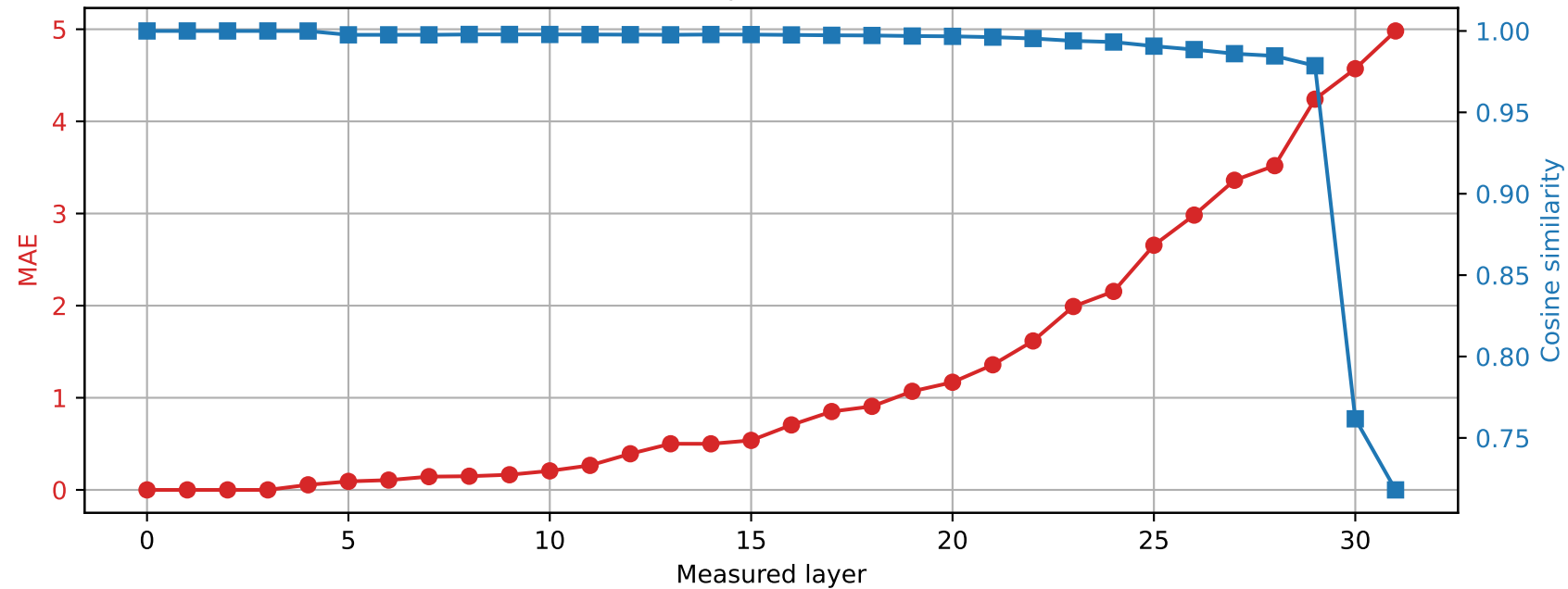
Phi-3-mini-4k-instruct | Prompt 3 Spared layer 3 | Hybrid vs quantized
