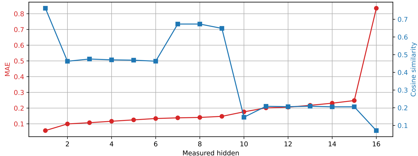
OLMo-1B-hf | Prompt 3 Spared layer 5 | Unquantized vs hybrid
