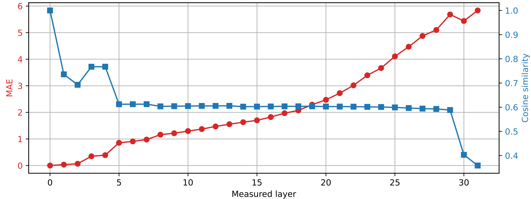
Phi-3-mini-4k-instruct | Prompt 3 Spared layer 9 | Hybrid vs unquantized
