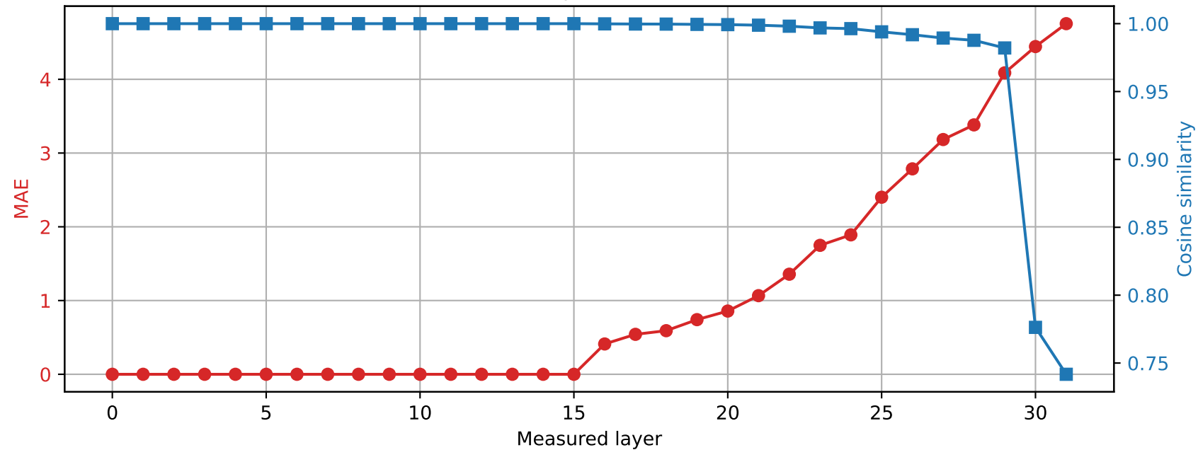
Phi-3-mini-4k-instruct | Prompt 3 Spared layer 15 | Hybrid vs quantized
