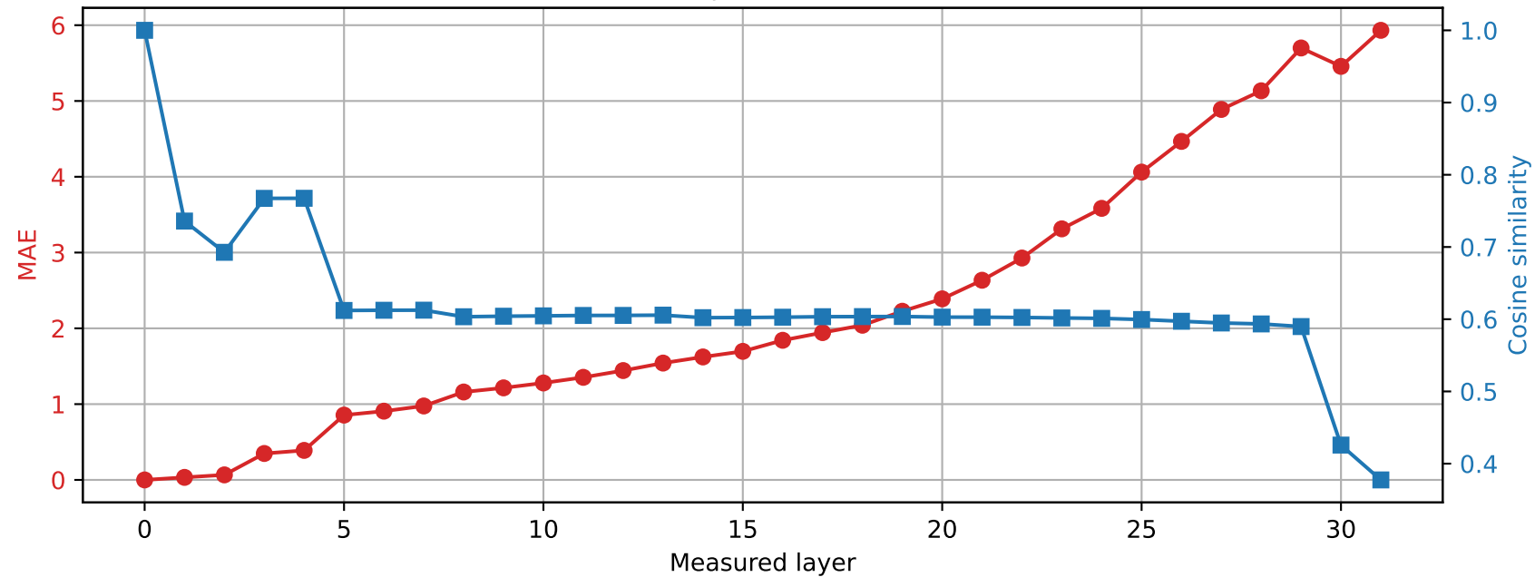
Phi-3-mini-4k-instruct | Prompt 3 Spared layer 16 | Hybrid vs unquantized
