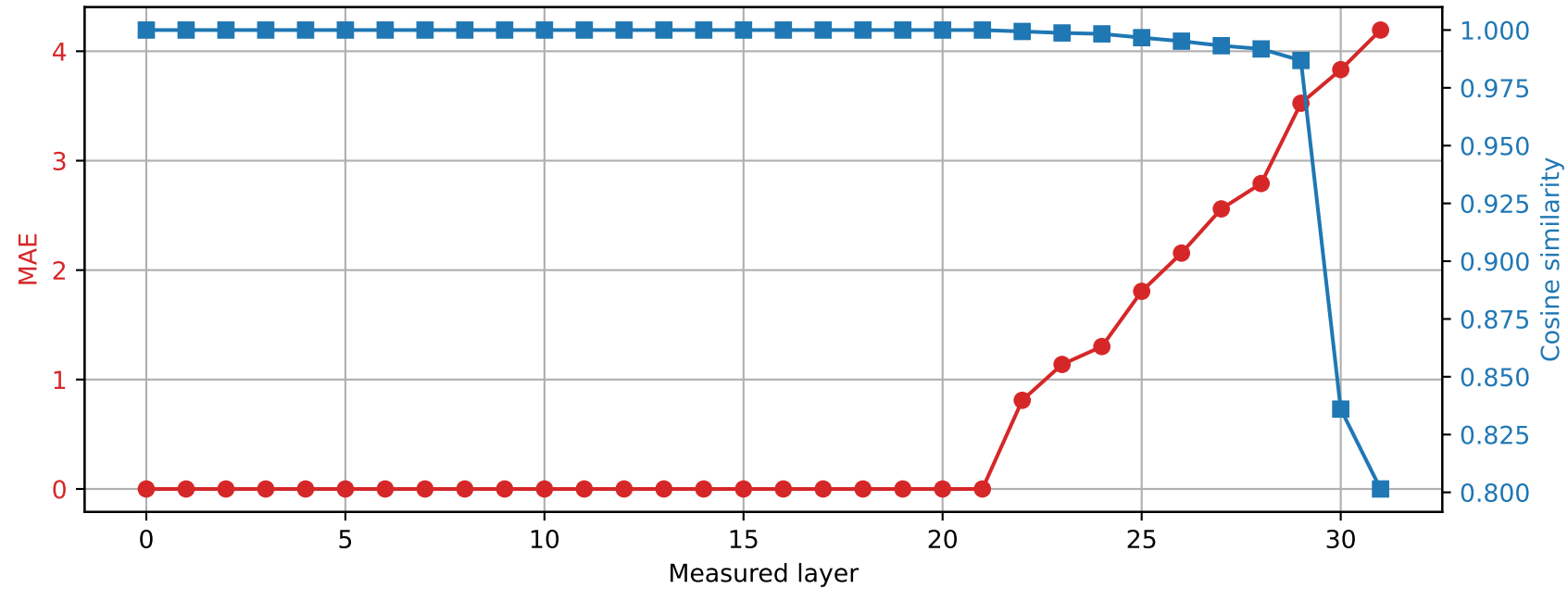
Phi-3-mini-4k-instruct | Prompt 3 Spared layer 21 | Hybrid vs quantized
