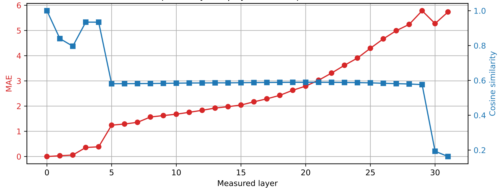
Phi-3-mini-4k-instruct | Prompt 4 Spared layer 2 | Hybrid vs unquantized
