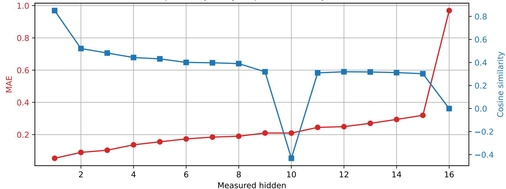
OLMo-1B-hf | Prompt 4 Spared layer 8 | Unquantized vs hybrid
