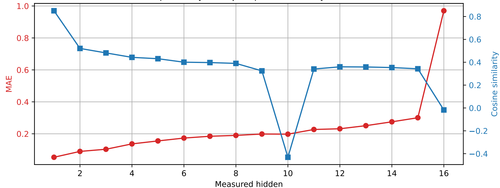
OLMo-1B-hf | Prompt 4 Spared layer 10 | Unquantized vs hybrid
