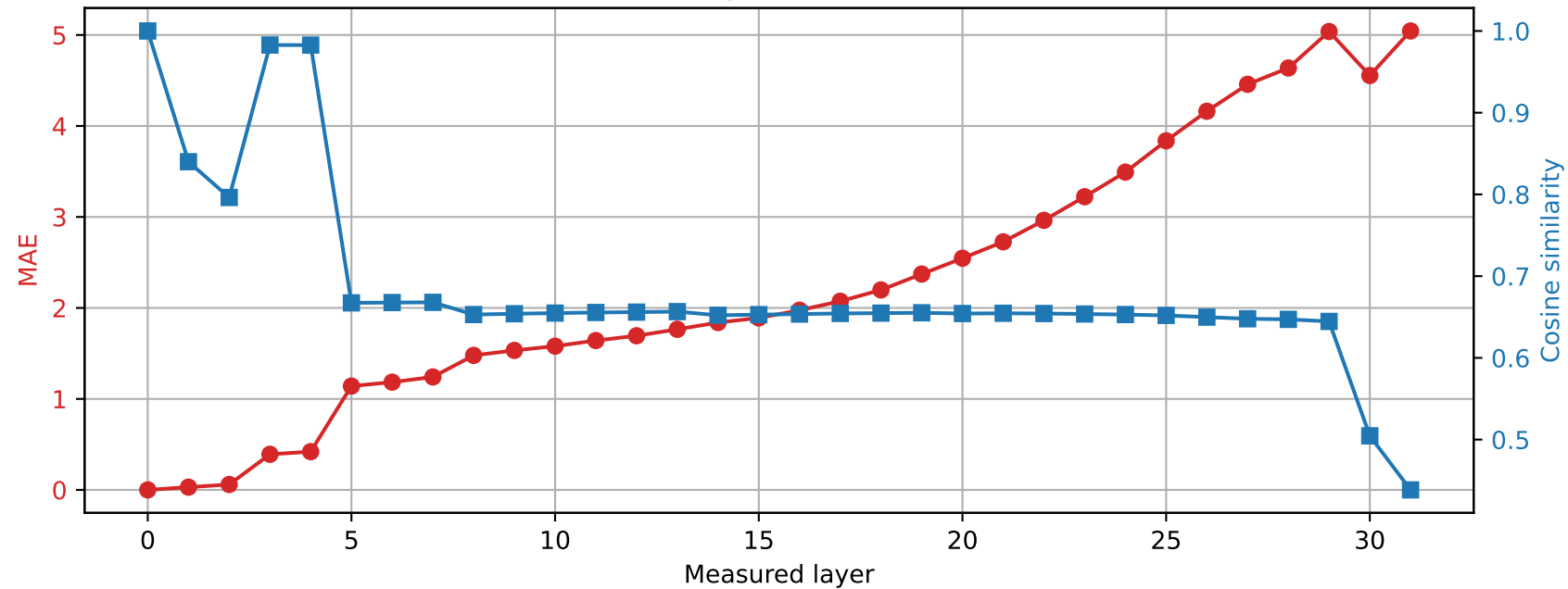
Phi-3-mini-4k-instruct | Prompt 4 Spared layer 19 | Hybrid vs unquantized
