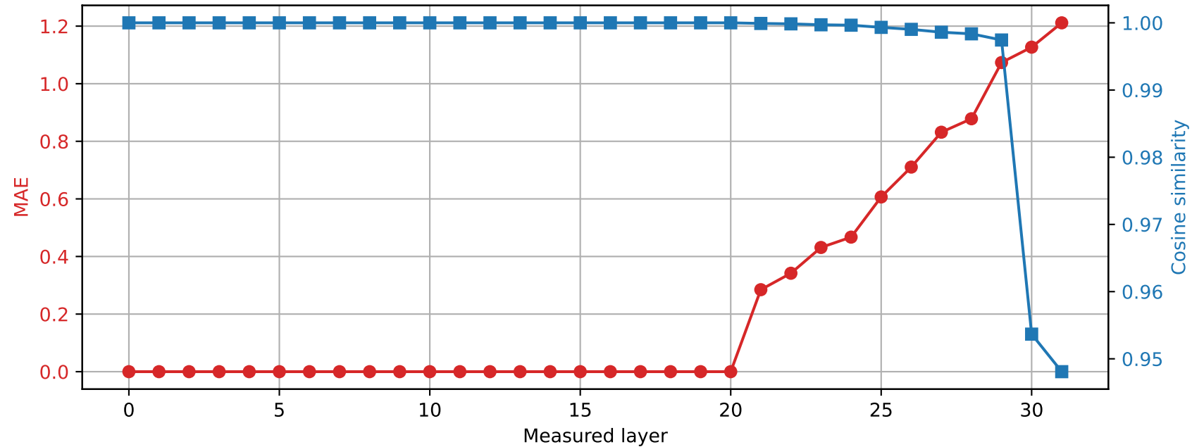
Phi-3-mini-4k-instruct | Prompt 4 Spared layer 20 | Hybrid vs quantized
